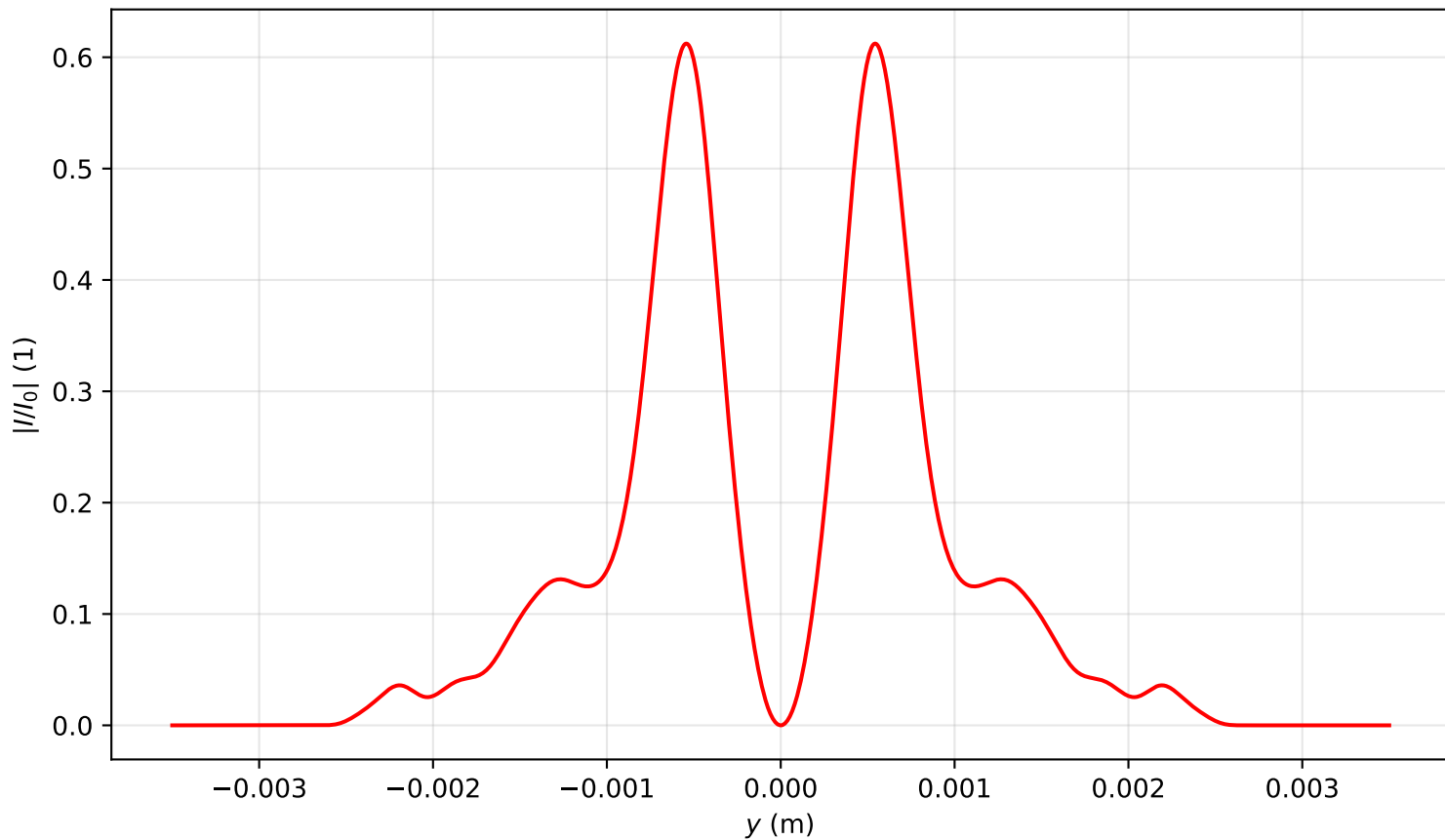
Intensity profile I(x=0, y, z=2.786)/I_0 , P_{in}=5.0P_{cr} , artificial time
